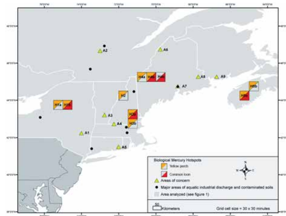
Figure 2. Distribution of biological mercury hotspots (H1a–H5b) and areas of concern (A1–A9). Areas of concern: A1, Catskill Mountains, New York; A2, LaMauricie region, Quebec, Canada; A3, Deerfield River, Vermont; A4, north-central Massachusetts; A5, lower Thames River, Connecticut; A6, upper St. John River, Maine; A7, lower Penobscot River, Maine; A8, Downeast region, Maine; A9, Lepreau region, New Brunswick, Canada. Hotspots: H1a, western Adirondack Mountains, New York; H1b, central Adirondack Mountains, New York; H2, upper Connecticut River, New Hampshire and Vermont; H3a, middle Merrimack River, New Hampshire; H3b, lower Merrimack River, Massachusetts and New Hampshire; H4a, upper Androscoggin River, Maine and New Hampshire; H4b, western upper Kennebec River, Maine; H4c, eastern upper Kennebec River, Maine; H5a, Kejimikujik National Park, Nova Scotia, Canada; H5b, central Nova Scotia.
