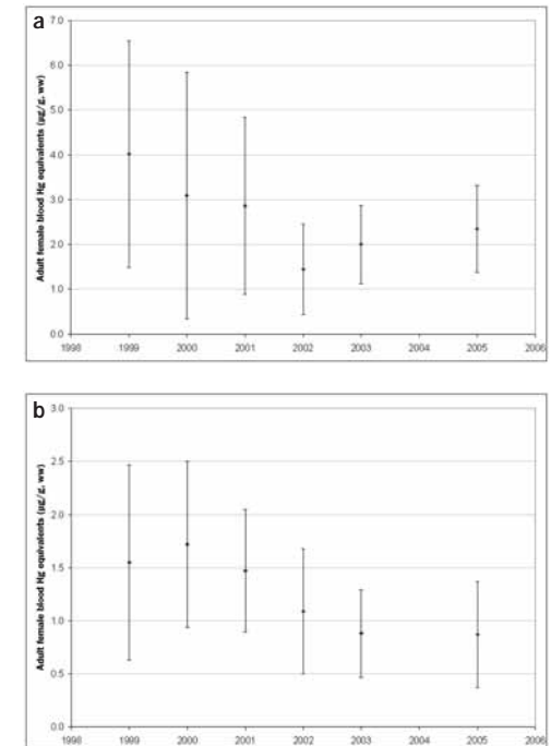
Figure 6. Temporal patterns for adult loon blood mercury (Hg) equivalents ( \mu\text{g per g} , wet weight; mean \pm standard deviation) in (a) the middle Merrimack River watershed ( n = 53 ) and (b) the upper Merrimack River watershed ( n = 43 ), New Hampshire. Note: The magnitude of the y axis, adult female blood Hg equivalents, differs between figure 6a and 6b.
