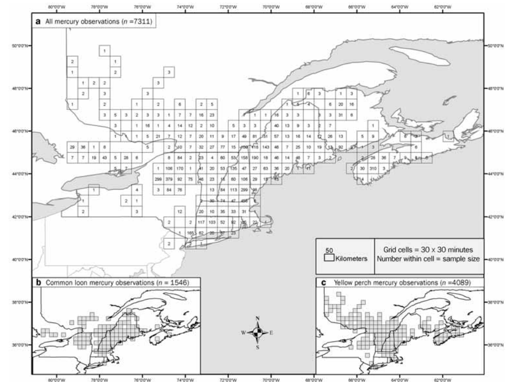
Figure 1. (a) Distribution of biotic mercury (Hg) observations across the northeastern United States and southeastern Canada, and specific distribution of Hg observations for (b) the common loon and (c) yellow perch.
