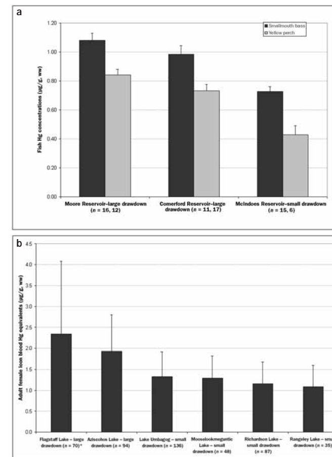
Figure 4. (a) Fillet mercury (Hg) concentrations for smallmouth bass and yellow perch (mean ± standard deviation [sd]) at three interconnected Connecticut River reservoirs in Vermont and New Hampshire and (b) blood Hg concentrations for the common loon (mean ± sd) at five interconnected Androscoggin River reservoirs in Maine and New Hampshire and one reservoir (Flagstaff Lake) in the upper Kennebec River watershed, Maine. (Although it is not hydrologically connected to the grid in the upper Androscoggin River watershed, Flagstaff Lake is illustrative of headwater reservoirs in that region that have large drawdowns.) Reservoir drawdowns from June through September that are less than 1 m are considered small, and those greater than 3 m are considered large. Kruskal-Wallis tests indicate significant differences between reservoirs with large and small drawdowns.
